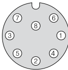
8-pin cable connector View on solder side
