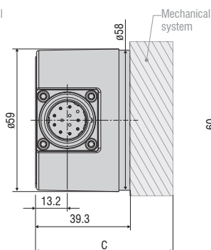
SSI output
