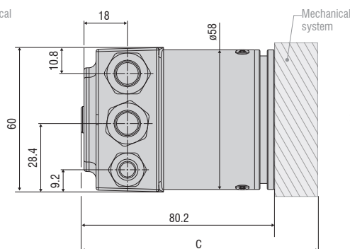
Output CO/PB
