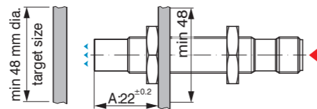
Fig. 4 Assembly, dimensions in mm (not to scale)
