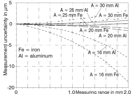
Fig. 5 Linearity deviation depending on distance A
