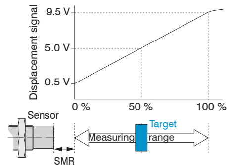
Fig. 3 Start of measuring range (SMR), the smallest distance between sensor face and measuring object
