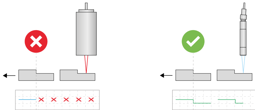
Conventional laser interferometer Reference required, loses position after signal interruption
